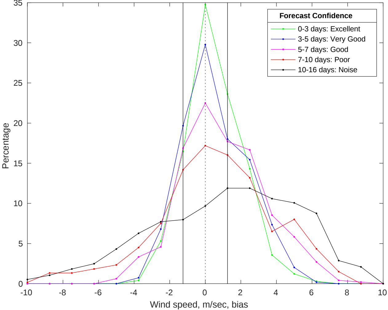
NDBC 46069 vs GFS Winds Bias Histogram: 07-Jul-2025
