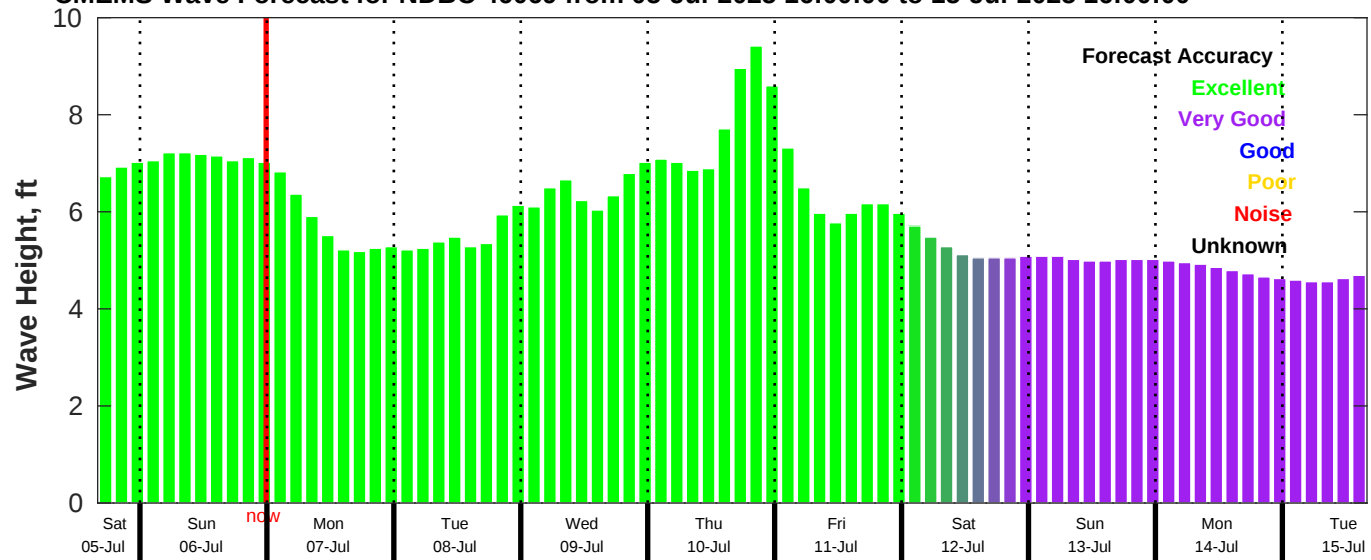
CMEMS Wave Forecast for NDBC 46069 from 05-Jul-2025 16:00:00 to 15-Jul-2025 16:00:00
