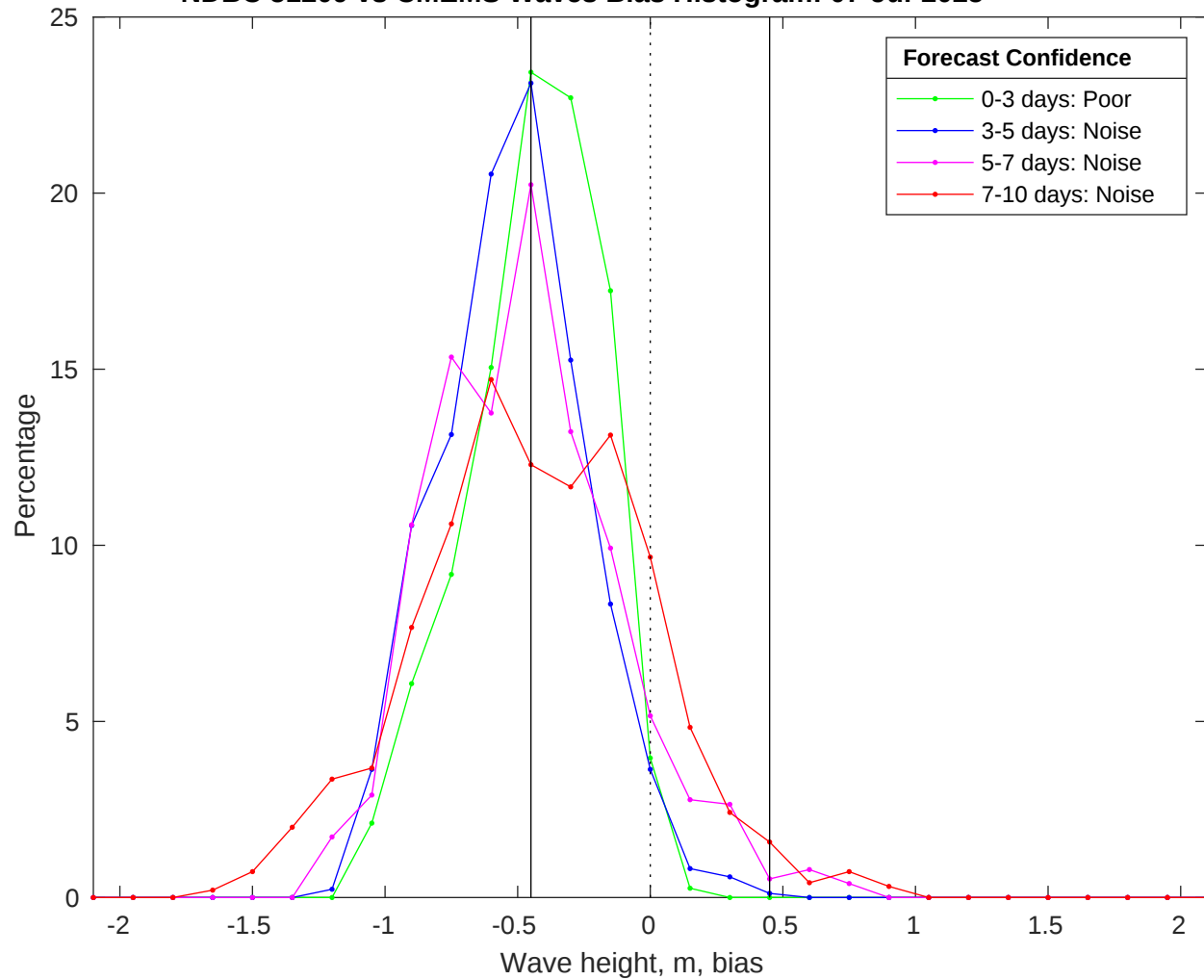
NDBC 51209 vs CMEMS Waves Bias Histogram: 07-Jul-2025
