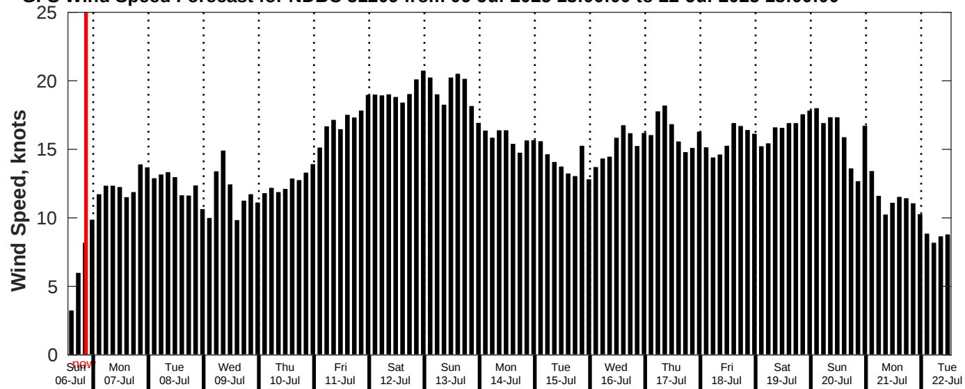
GFS Wind Speed Forecast for NDBC 51209 from 06-Jul-2025 13:00:00 to 22-Jul-2025 13:00:00
