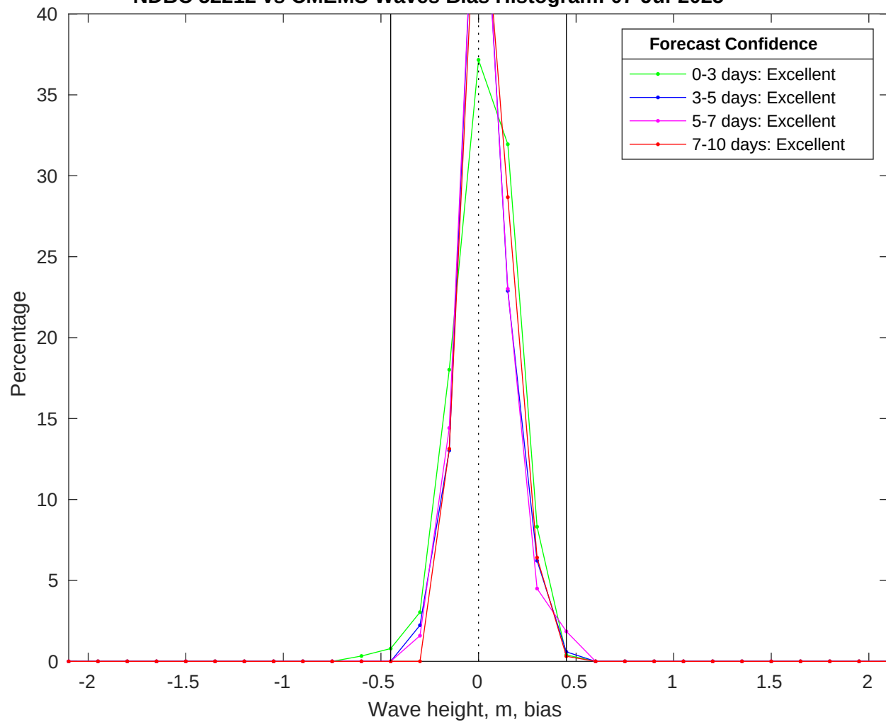
NDBC 52212 vs CMEMS Waves Bias Histogram: 07-Jul-2025
