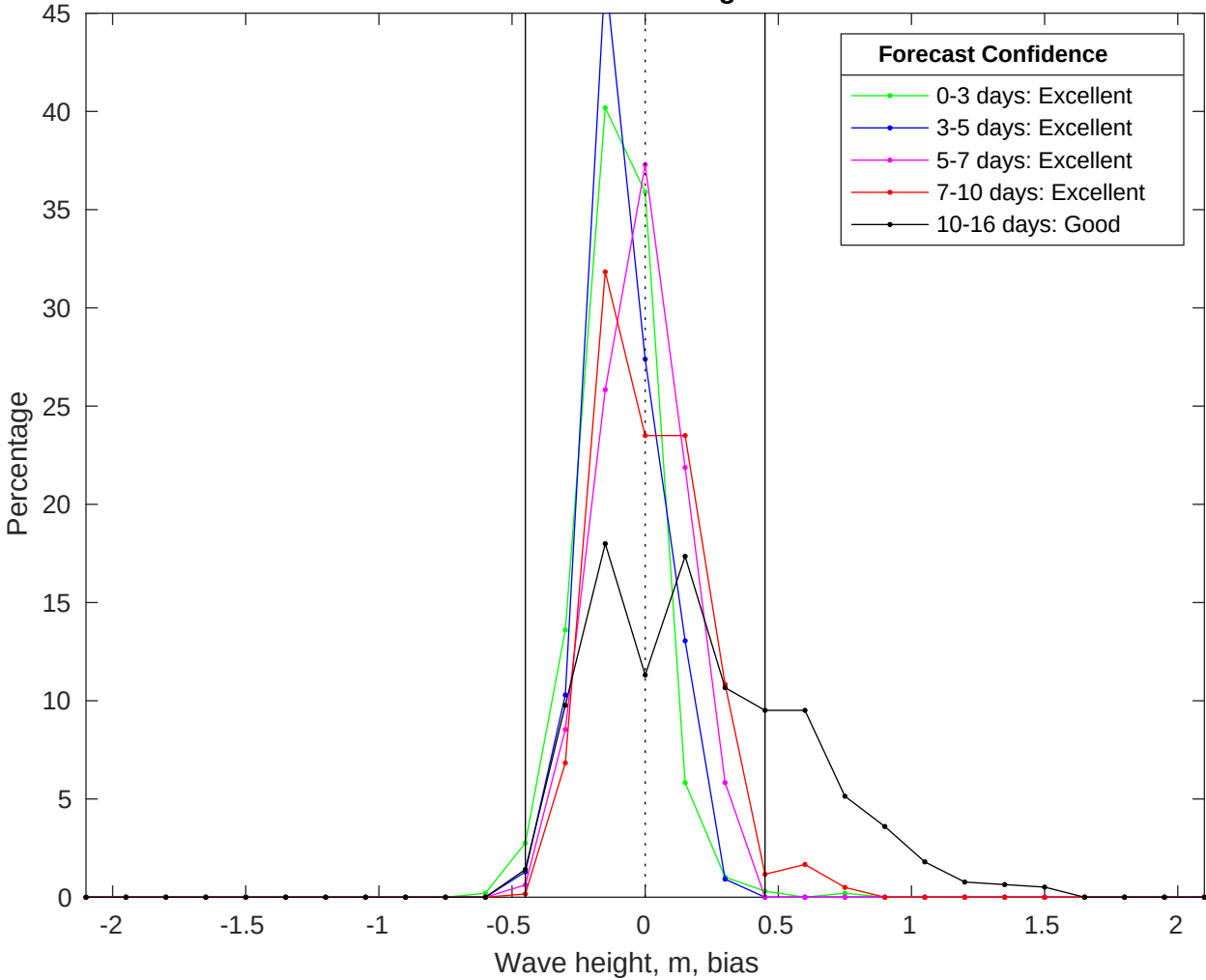
NDBC 52212 vs GFS Waves Bias Histogram: 07-Jul-2025
