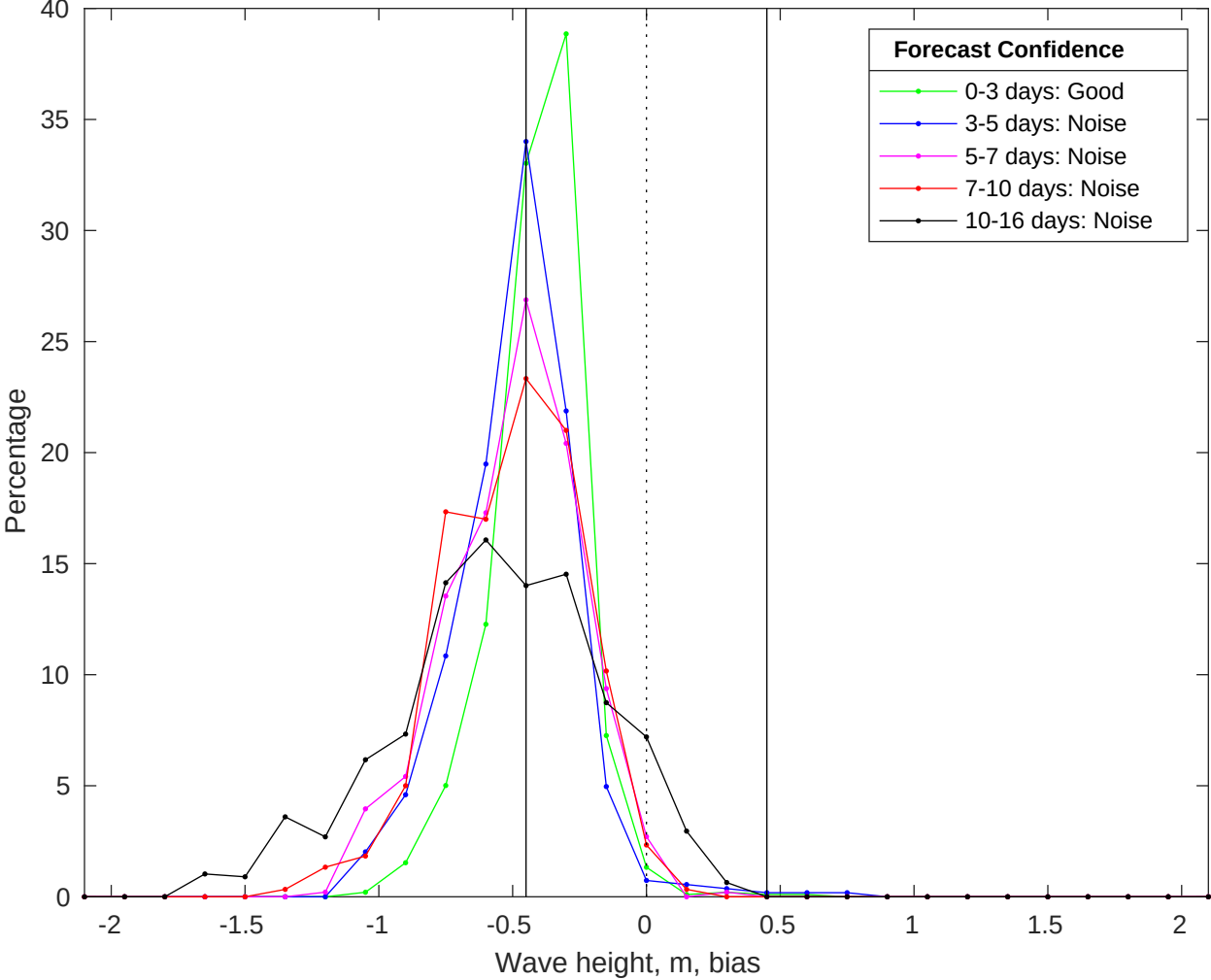
NDBC 52213 vs GFS Waves Bias Histogram: 07-Jul-2025
