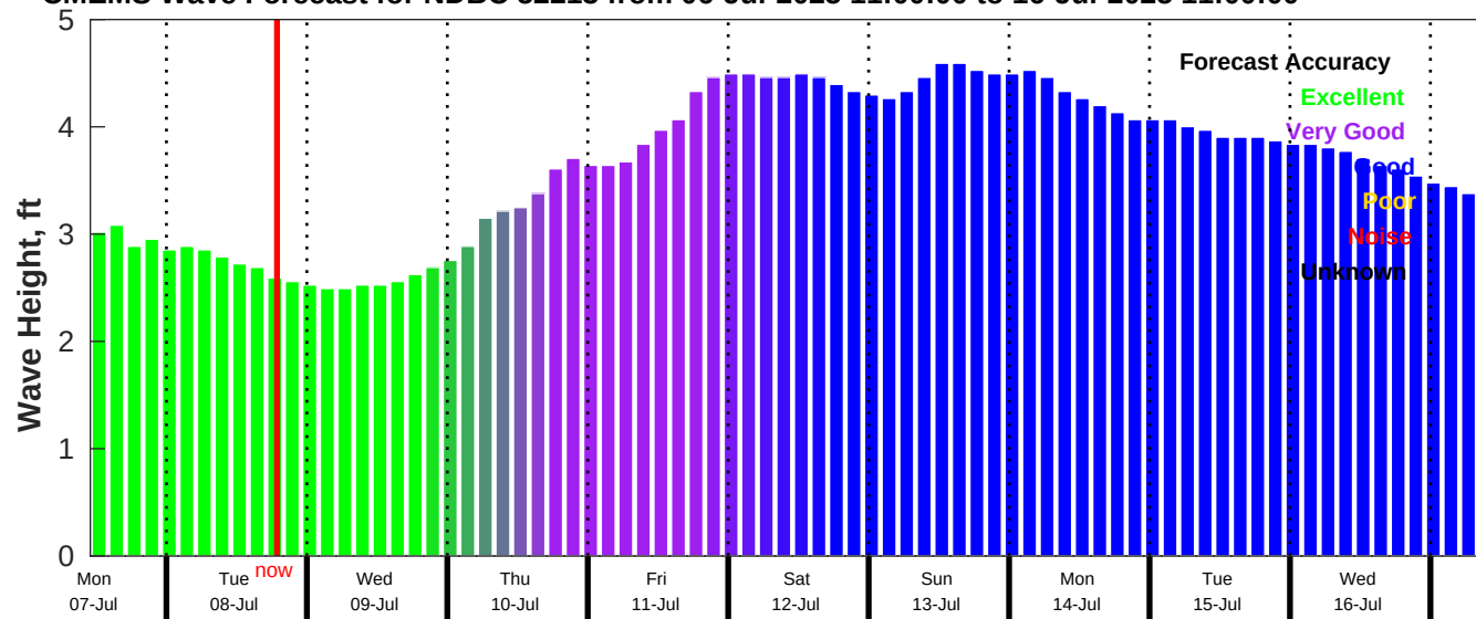
CMEMS Wave Forecast for NDBC 52213 from 06-Jul-2025 11:00:00 to 16-Jul-2025 11:00:00
