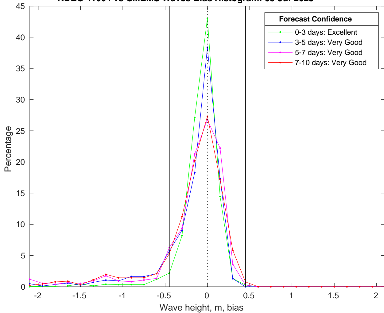
NDBC 41004 vs CMEMS Waves Bias Histogram: 08-Jul-2025
