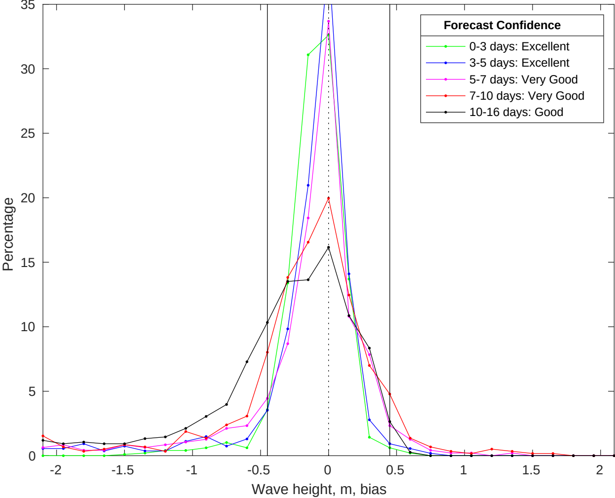
NDBC 41004 vs GFS Waves Bias Histogram: 08-Jul-2025
