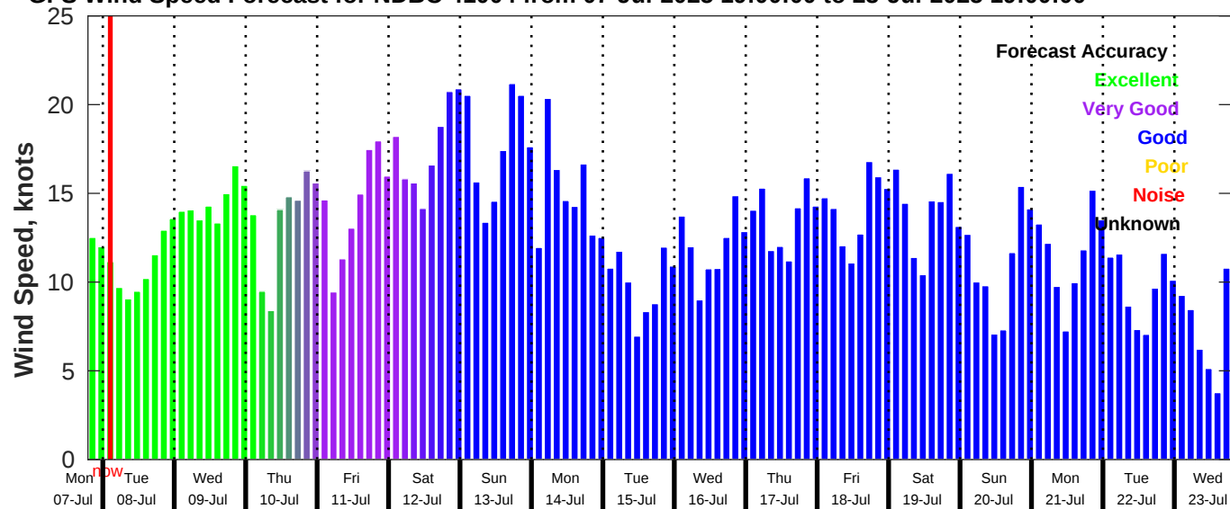
GFS Wind Speed Forecast for NDBC 41004 from 07-Jul-2025 19:00:00 to 23-Jul-2025 19:00:00
