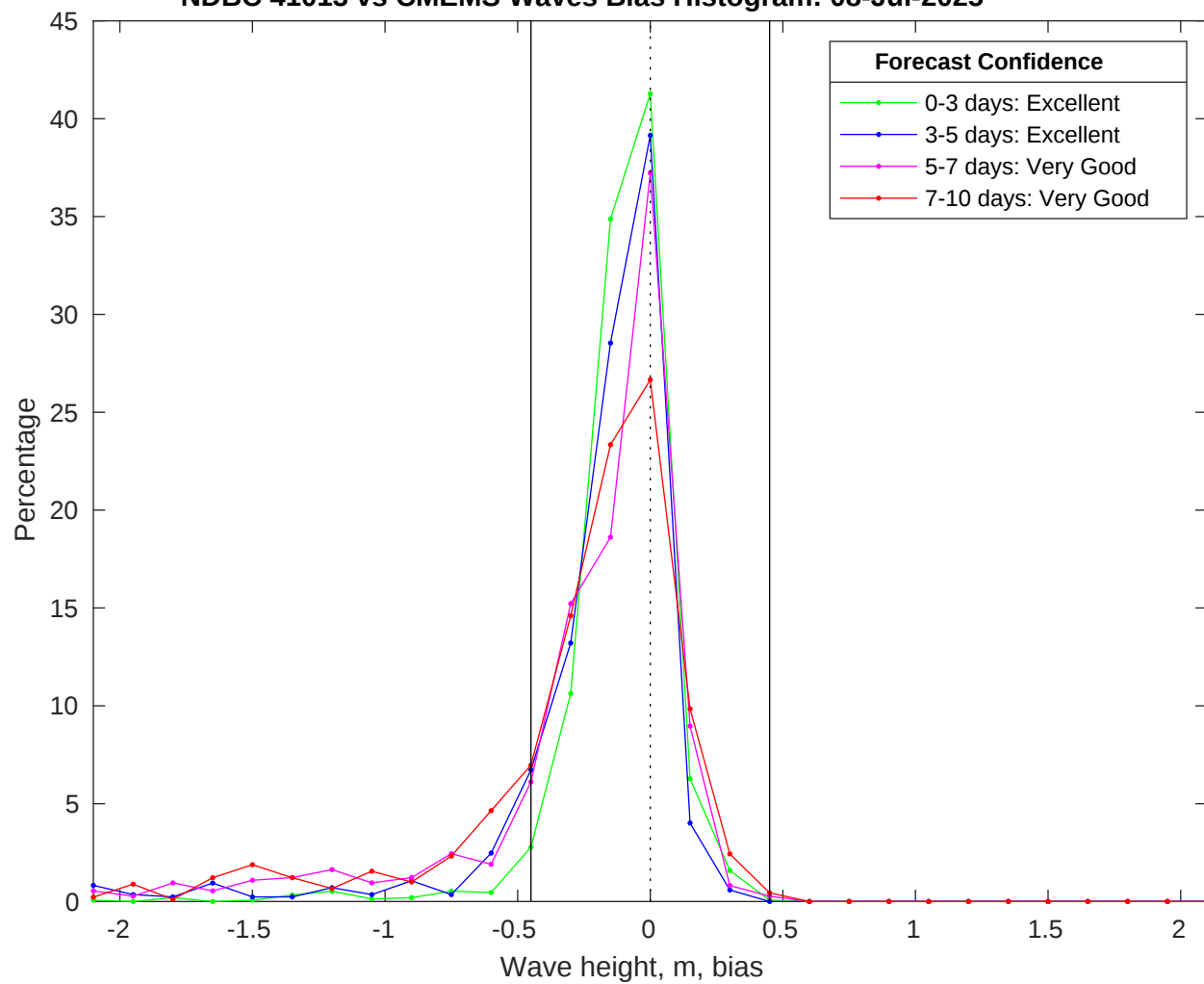
NDBC 41013 vs CMEMS Waves Bias Histogram: 08-Jul-2025
