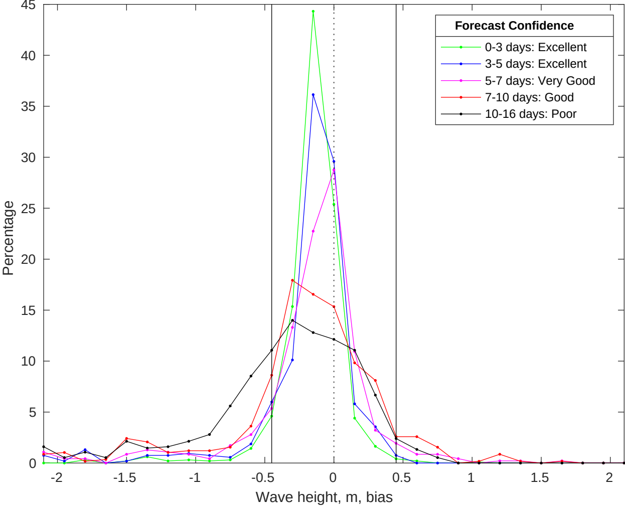
NDBC 41013 vs GFS Waves Bias Histogram: 08-Jul-2025
