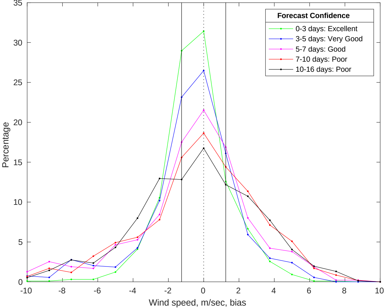
NDBC 41013 vs GFS Winds Bias Histogram: 08-Jul-2025
