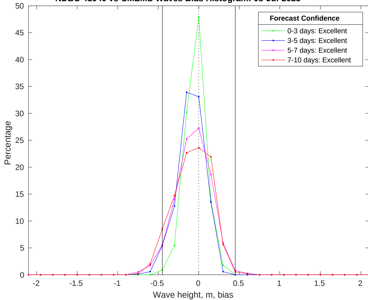
NDBC 41040 vs CMEMS Waves Bias Histogram: 08-Jul-2025
