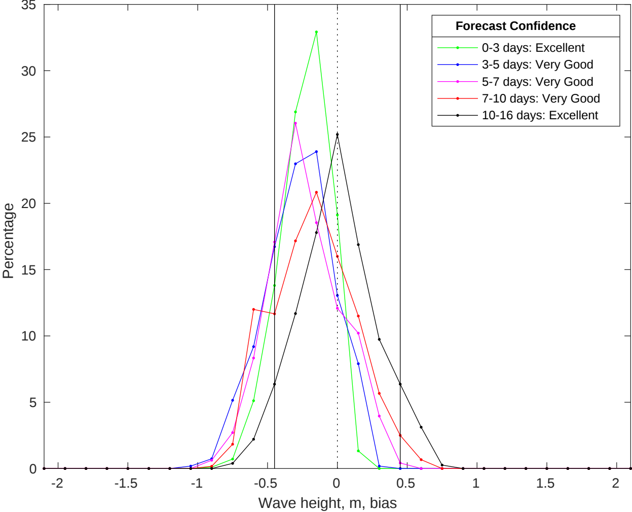
NDBC 41040 vs GFS Waves Bias Histogram: 08-Jul-2025
