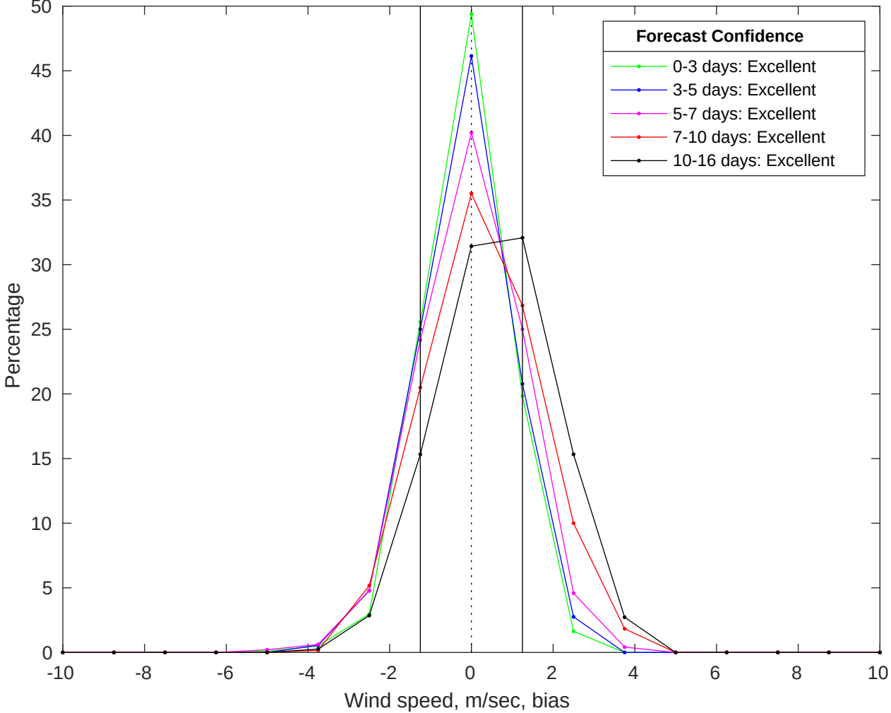
NDBC 41040 vs GFS Winds Bias Histogram: 08-Jul-2025
