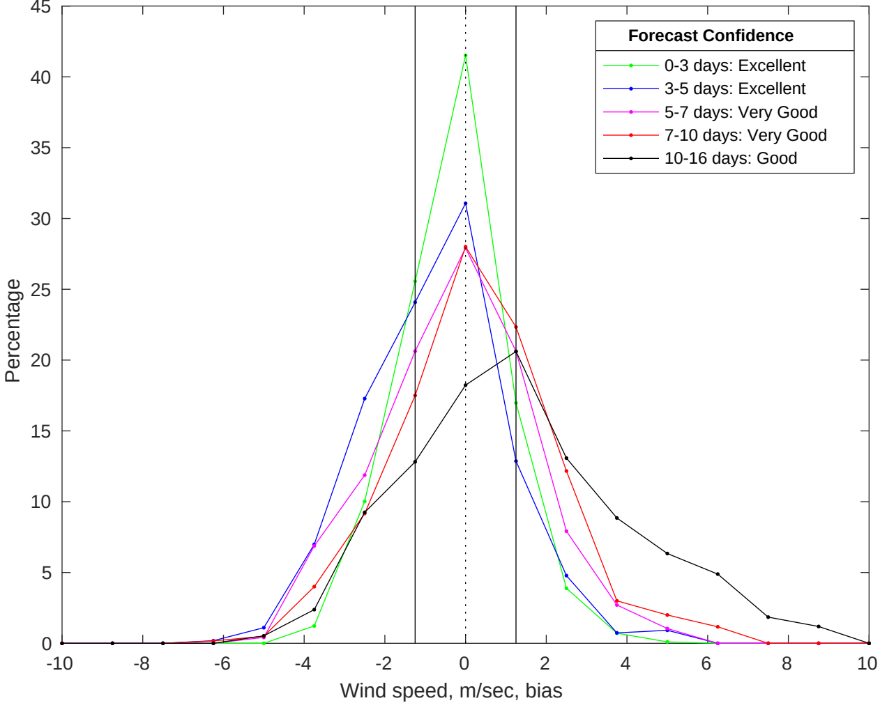
NDBC 42019 vs GFS Winds Bias Histogram: 08-Jul-2025
