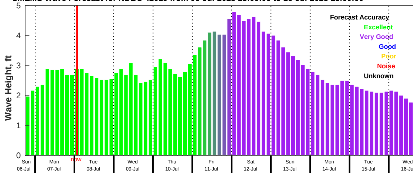
CMEMS Wave Forecast for NDBC 42019 from 06-Jul-2025 18:00:00 to 16-Jul-2025 18:00:00
