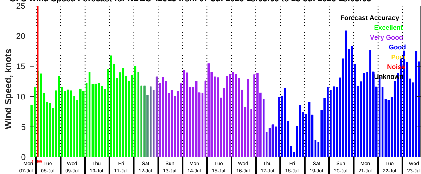
GFS Wind Speed Forecast for NDBC 42019 from 07-Jul-2025 18:00:00 to 23-Jul-2025 18:00:00
