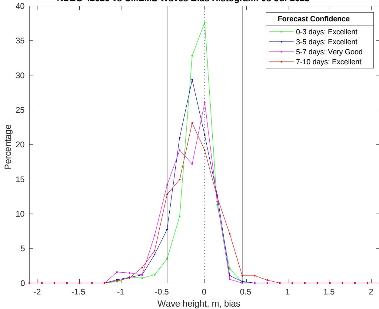
NDBC 42020 vs CMEMS Waves Bias Histogram: 08-Jul-2025
