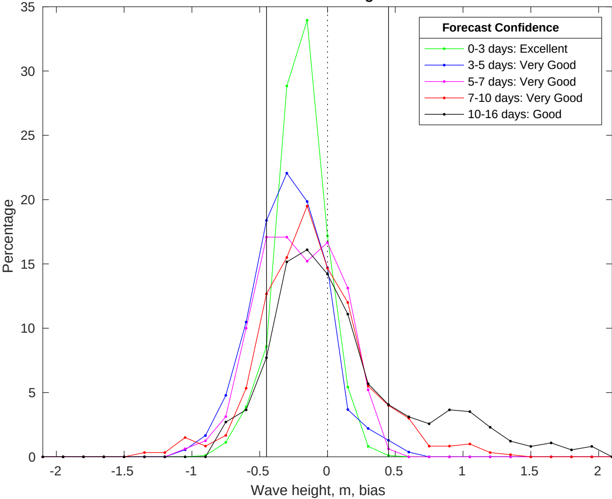
NDBC 42020 vs GFS Waves Bias Histogram: 08-Jul-2025
