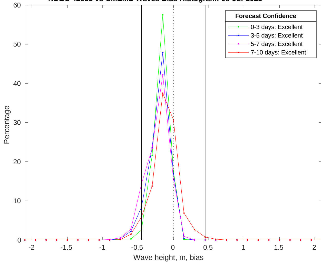
NDBC 42035 vs CMEMS Waves Bias Histogram: 08-Jul-2025
