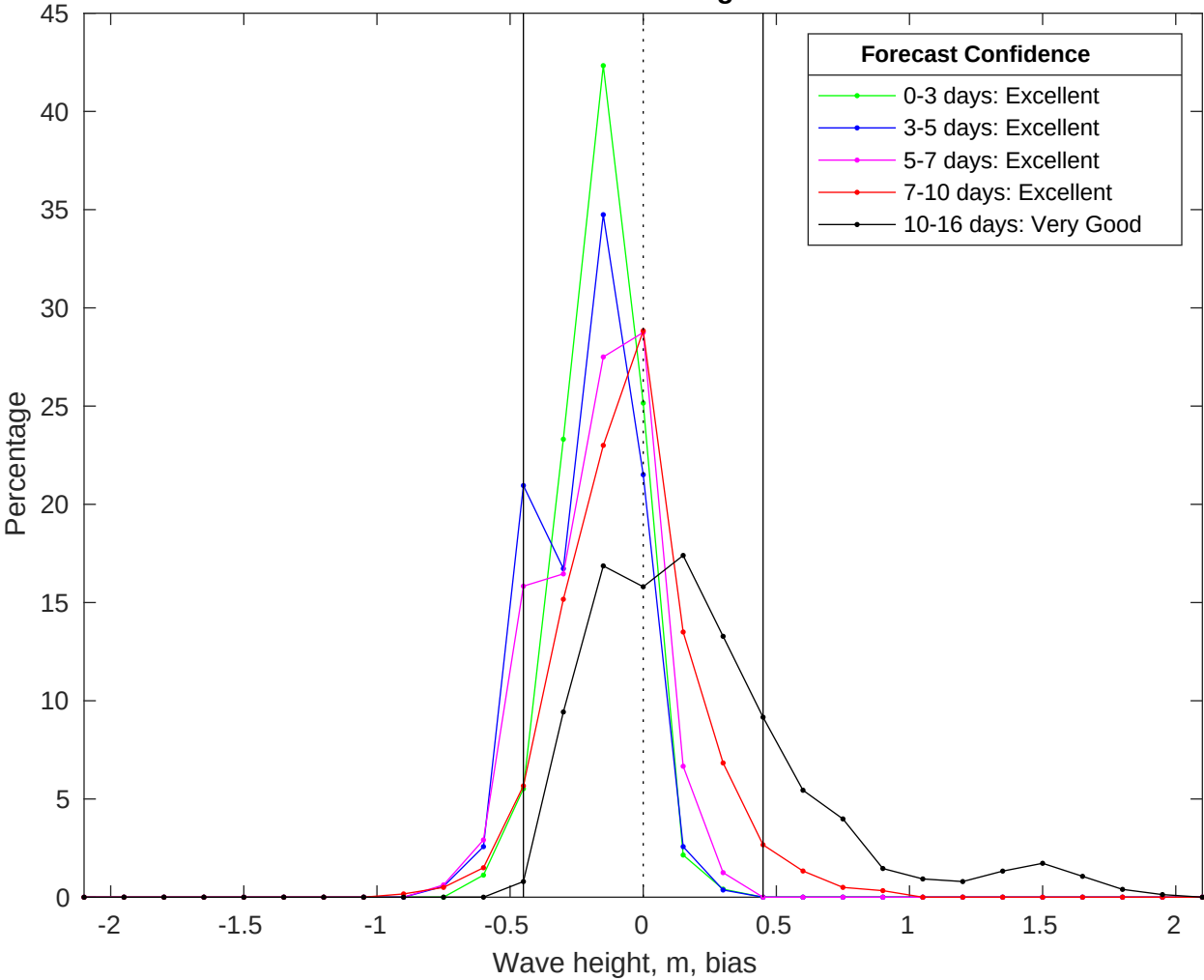
NDBC 42035 vs GFS Waves Bias Histogram: 08-Jul-2025
