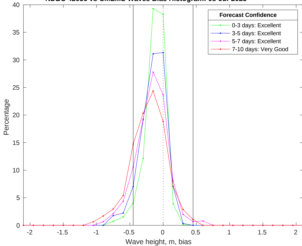
NDBC 42036 vs CMEMS Waves Bias Histogram: 08-Jul-2025
