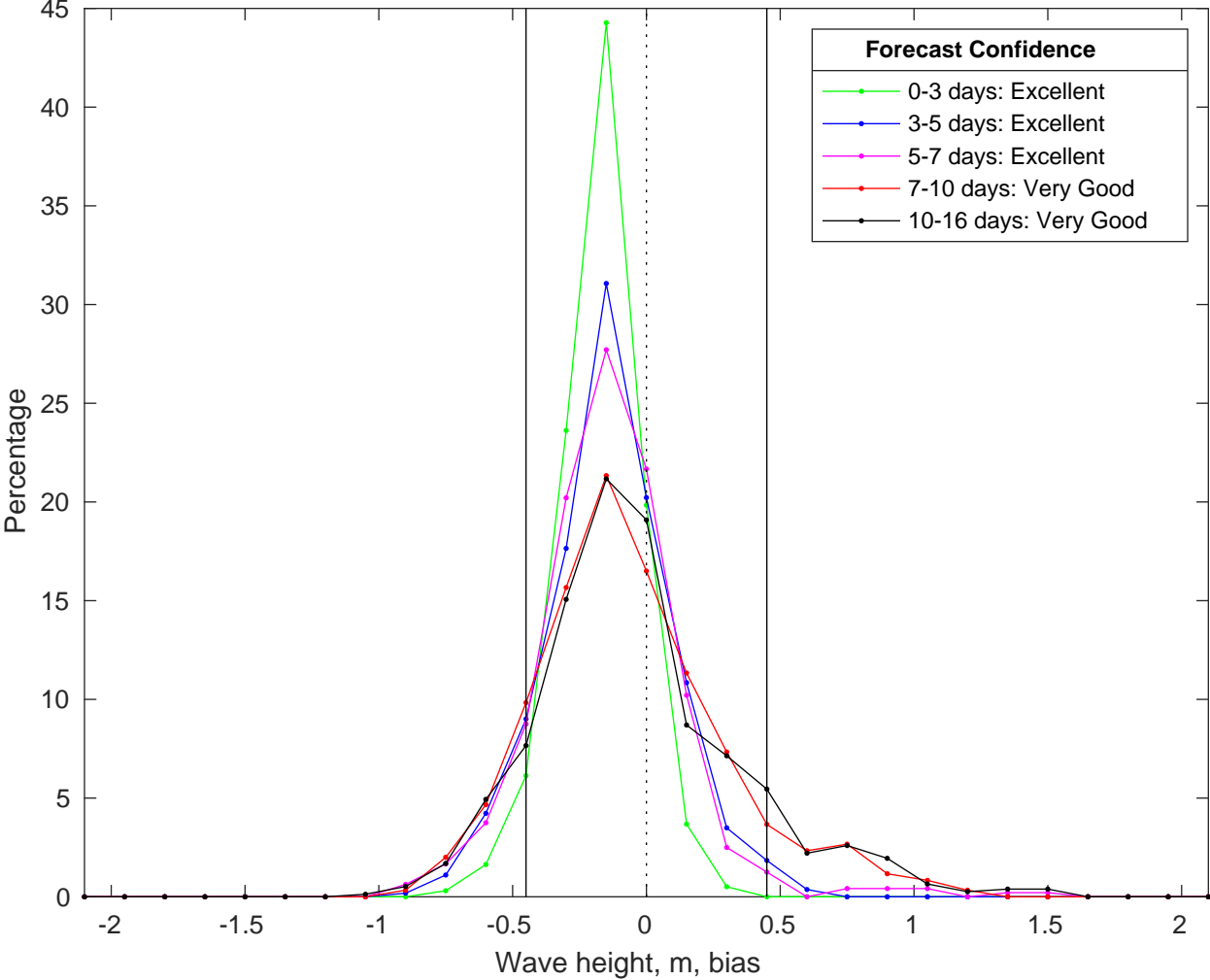
NDBC 42036 vs GFS Waves Bias Histogram: 08-Jul-2025
