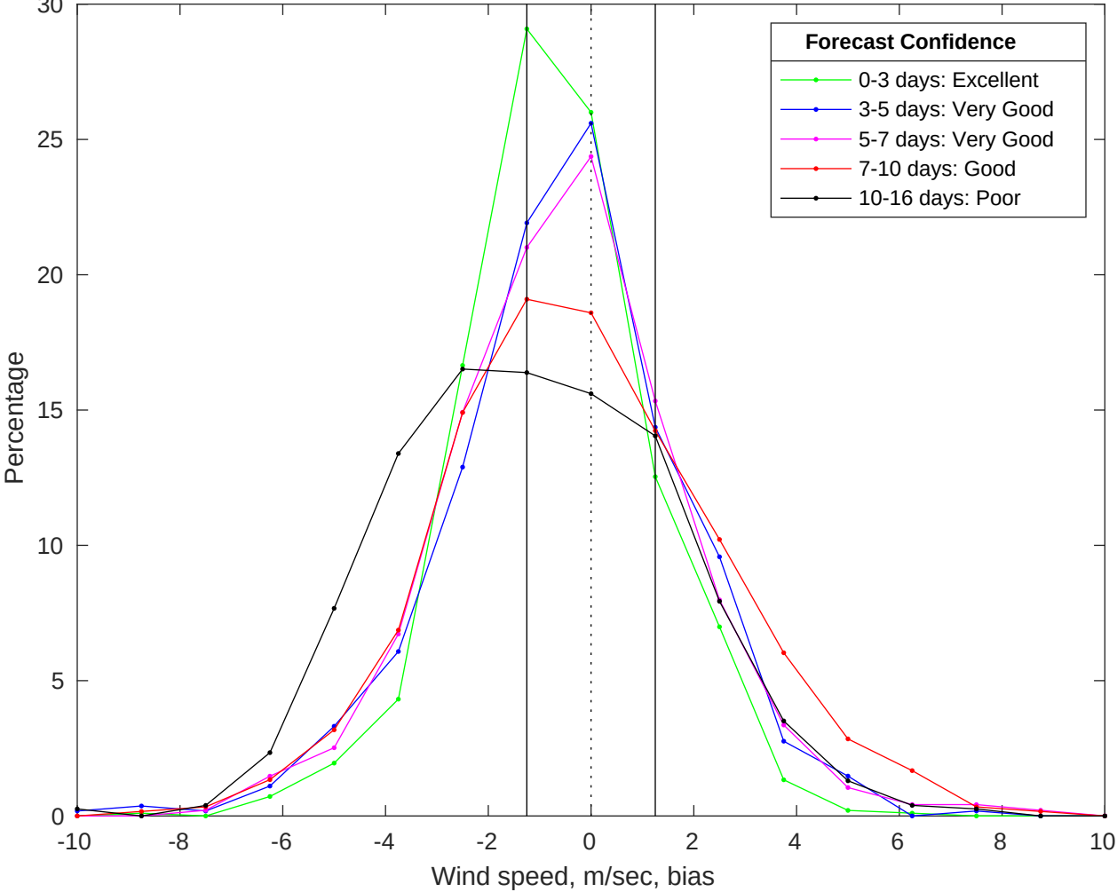
NDBC 42036 vs GFS Winds Bias Histogram: 08-Jul-2025
