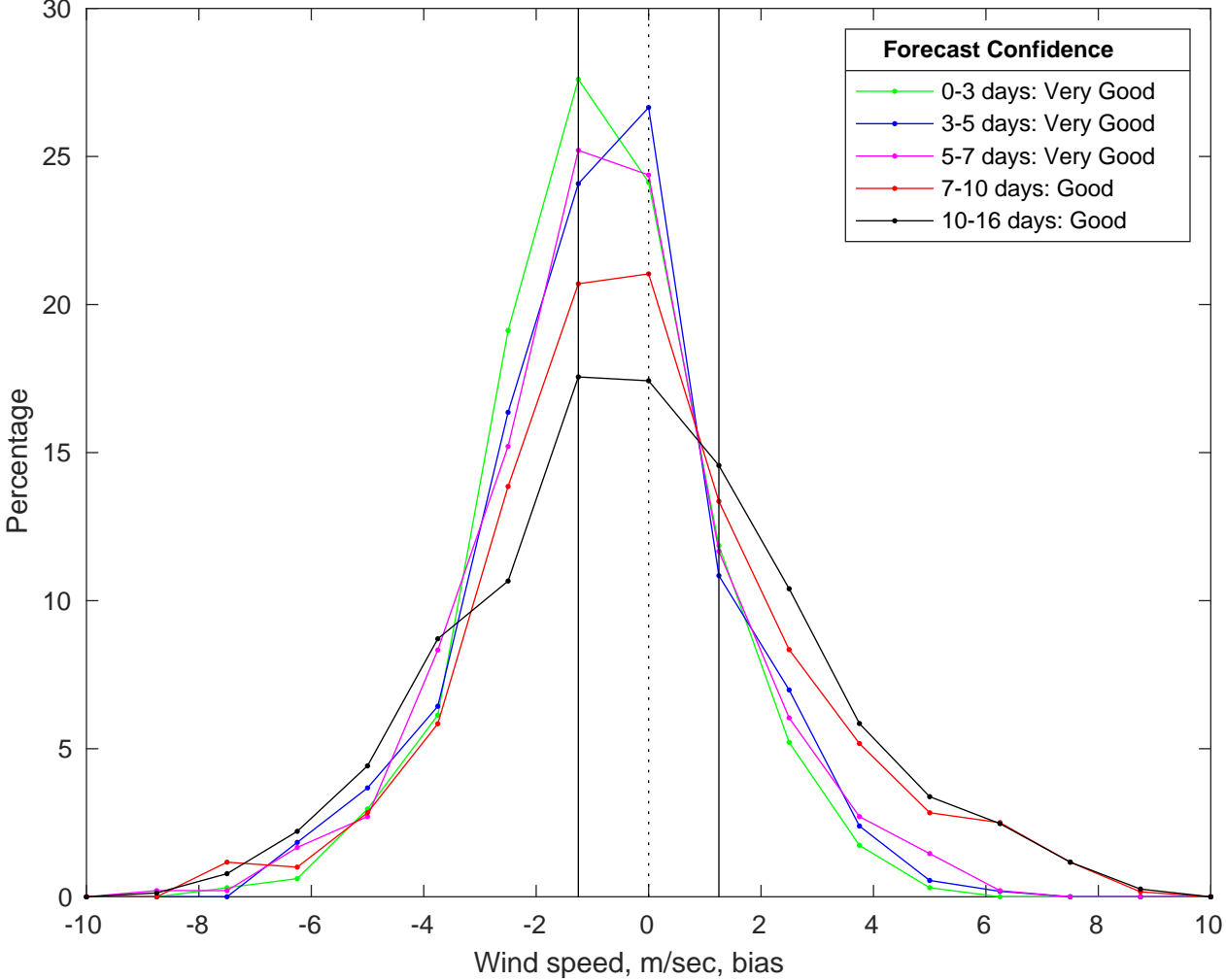
NDBC 42040 vs GFS Winds Bias Histogram: 08-Jul-2025
