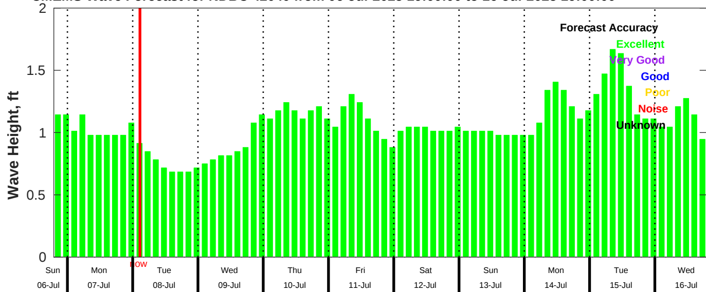
CMEMS Wave Forecast for NDBC 42040 from 06-Jul-2025 19:00:00 to 16-Jul-2025 19:00:00
