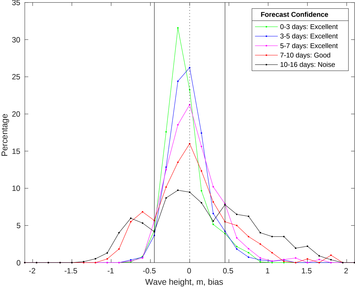
NDBC 46011 vs GFS Waves Bias Histogram: 08-Jul-2025
