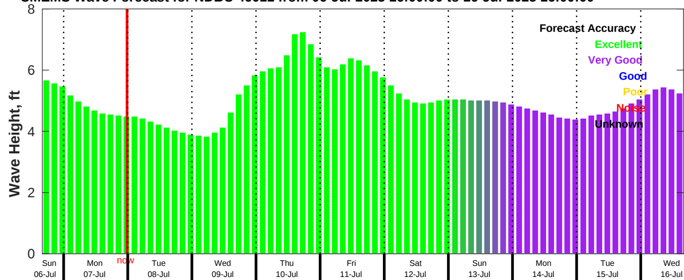
CMEMS Wave Forecast for NDBC 46011 from 06-Jul-2025 16:00:00 to 16-Jul-2025 16:00:00
