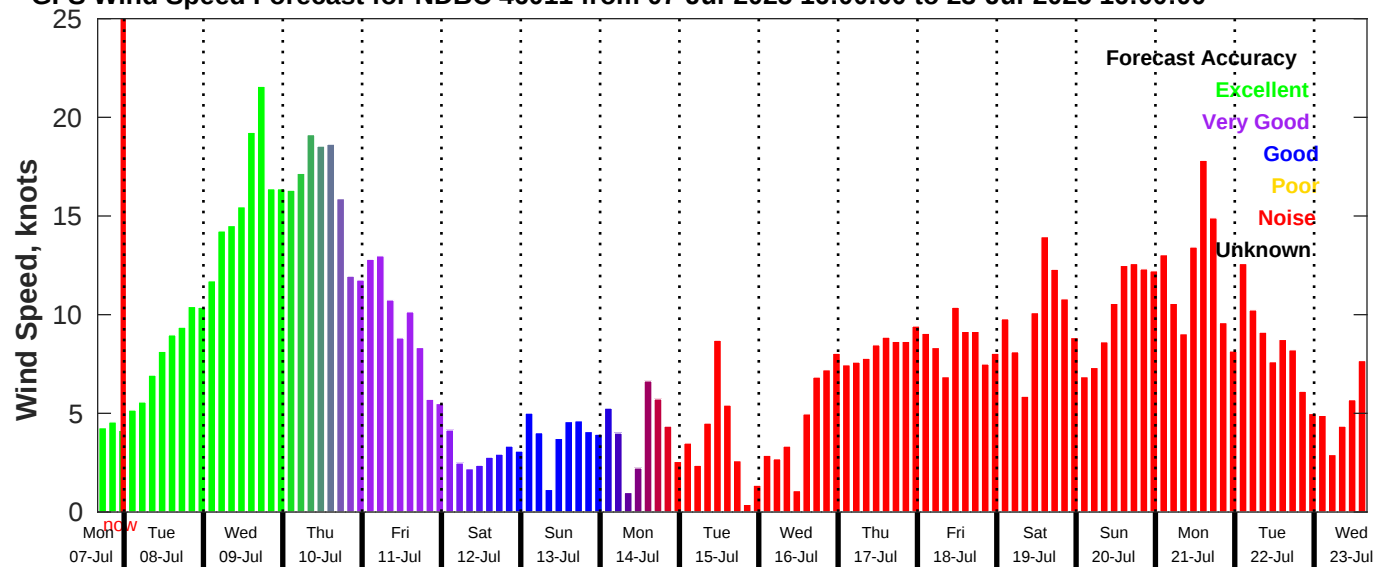
GFS Wind Speed Forecast for NDBC 46011 from 07-Jul-2025 16:00:00 to 23-Jul-2025 16:00:00
