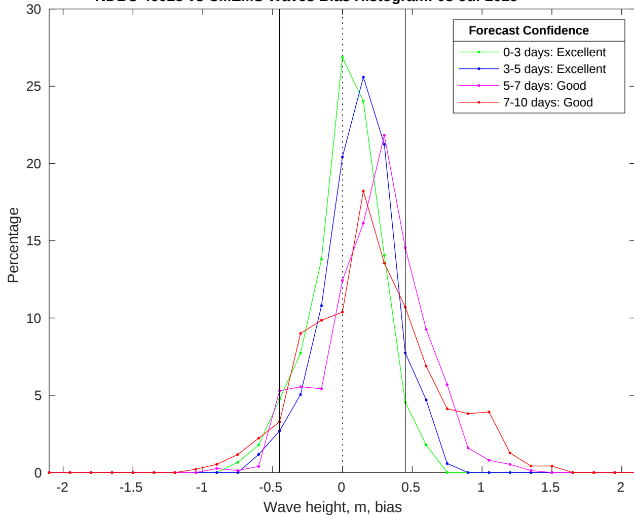
NDBC 46028 vs CMEMS Waves Bias Histogram: 08-Jul-2025
