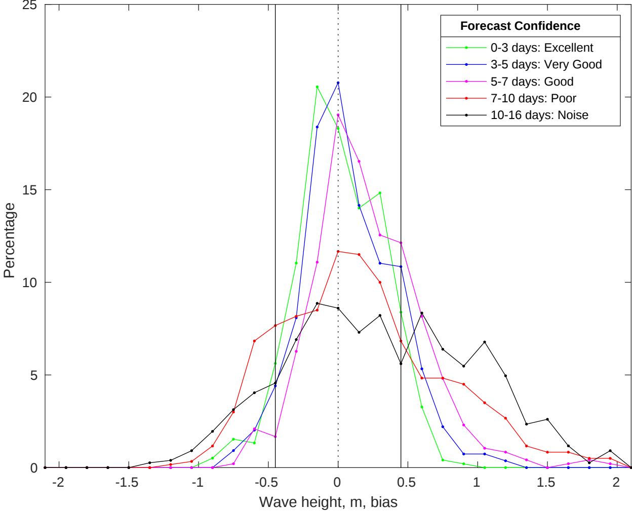
NDBC 46028 vs GFS Waves Bias Histogram: 08-Jul-2025
