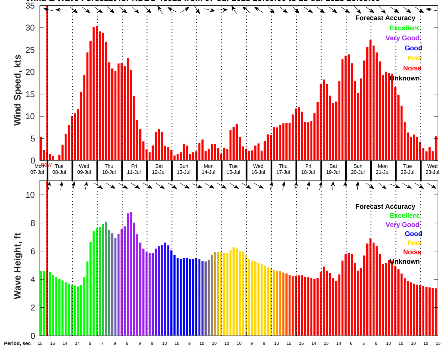
Wind & Wave Forecast for NDBC 46028 from 07-Jul-2025 16:00:00 to 23-Jul-2025 16:00:00
