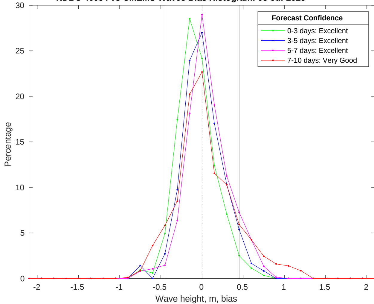
NDBC 46054 vs CMEMS Waves Bias Histogram: 08-Jul-2025
