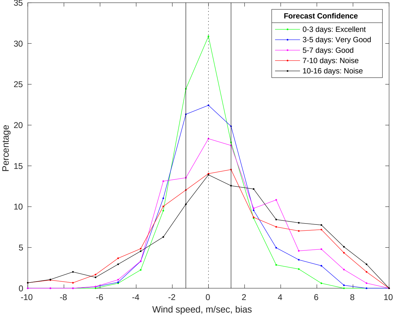
NDBC 46054 vs GFS Winds Bias Histogram: 08-Jul-2025
