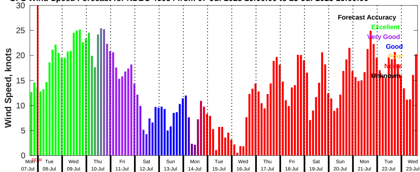
GFS Wind Speed Forecast for NDBC 46054 from 07-Jul-2025 16:00:00 to 23-Jul-2025 16:00:00
