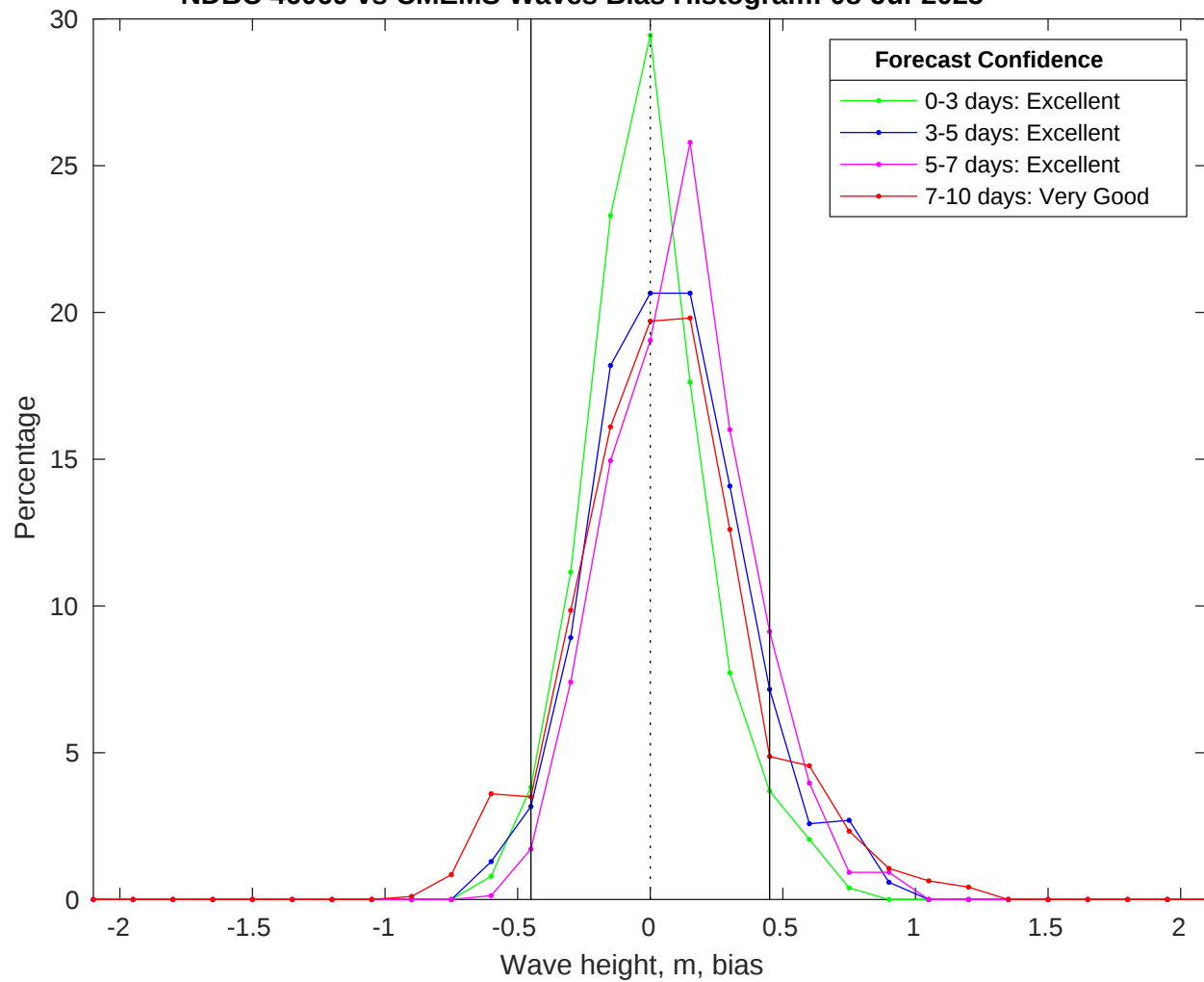
NDBC 46069 vs CMEMS Waves Bias Histogram: 08-Jul-2025
