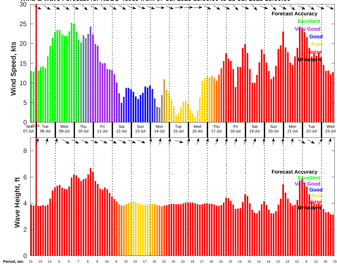
Wind & Wave Forecast for NDBC 46069 from 07-Jul-2025 16:00:00 to 23-Jul-2025 16:00:00
