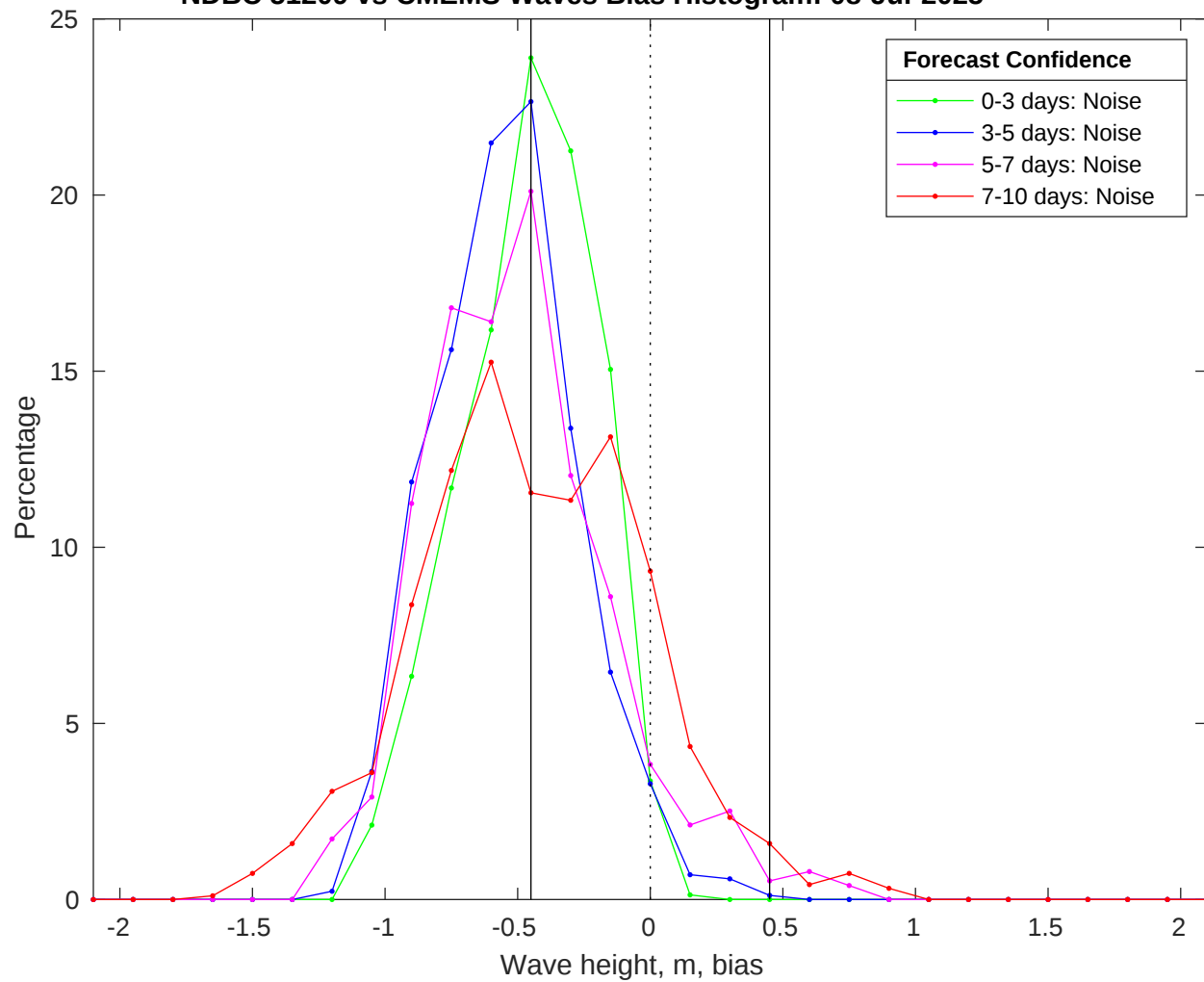
NDBC 51209 vs CMEMS Waves Bias Histogram: 08-Jul-2025
