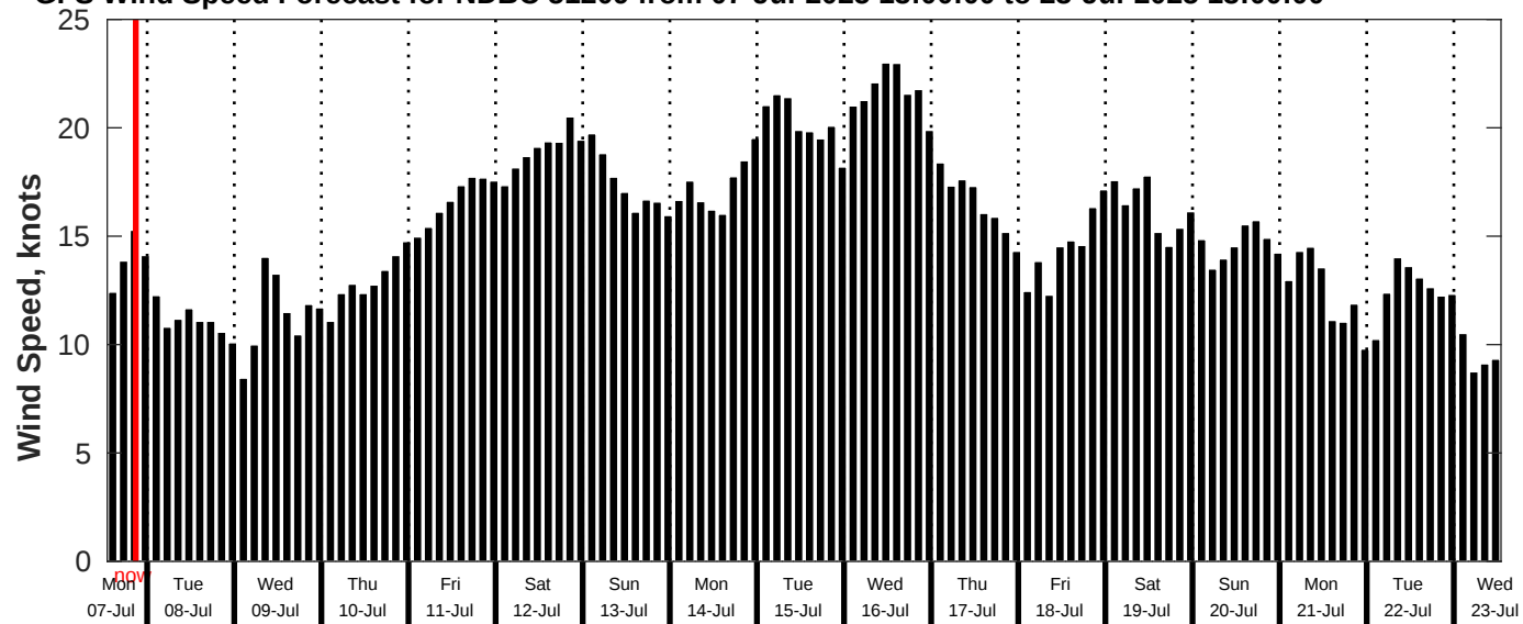
GFS Wind Speed Forecast for NDBC 51209 from 07-Jul-2025 13:00:00 to 23-Jul-2025 13:00:00
