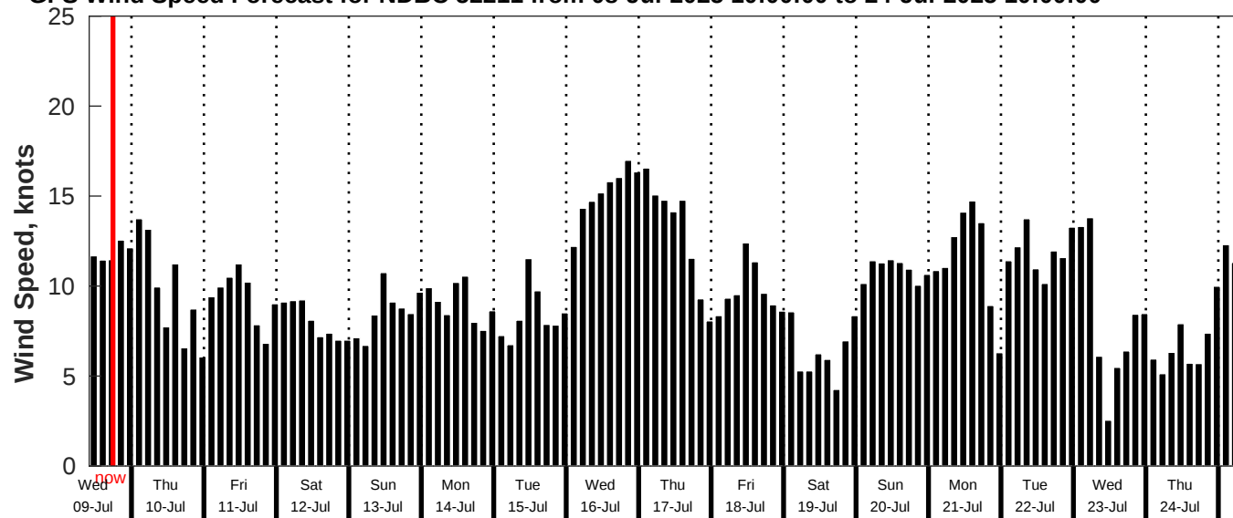
GFS Wind Speed Forecast for NDBC 52211 from 08-Jul-2025 10:00:00 to 24-Jul-2025 10:00:00
