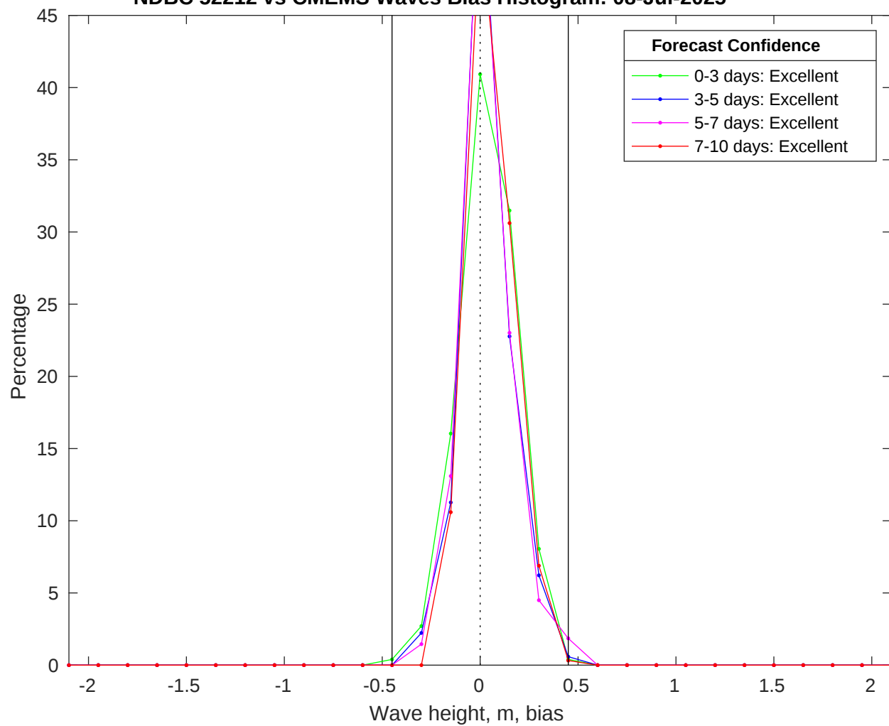
NDBC 52212 vs CMEMS Waves Bias Histogram: 08-Jul-2025
