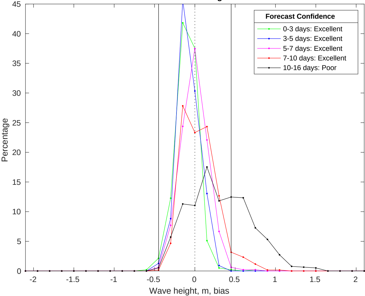
NDBC 52212 vs GFS Waves Bias Histogram: 08-Jul-2025
