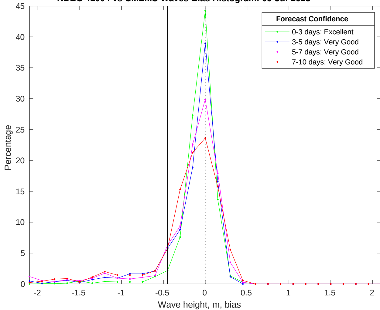
NDBC 41004 vs CMEMS Waves Bias Histogram: 09-Jul-2025
