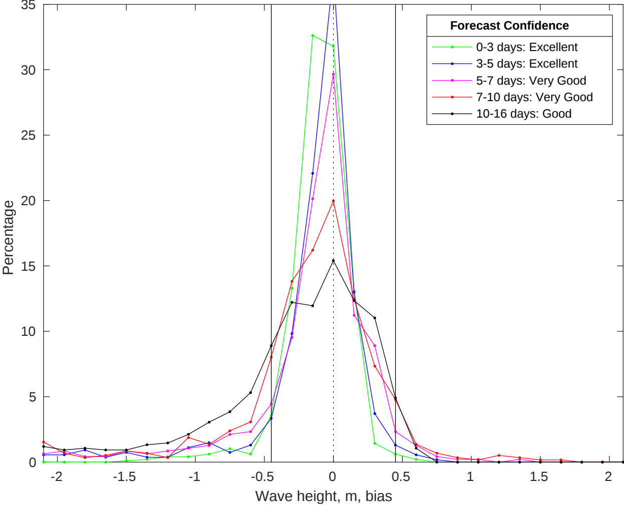
NDBC 41004 vs GFS Waves Bias Histogram: 09-Jul-2025
