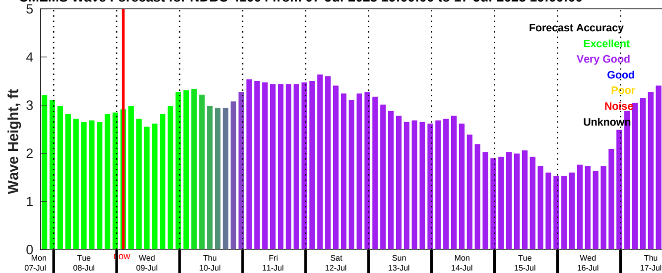
CMEMS Wave Forecast for NDBC 41004 from 07-Jul-2025 19:00:00 to 17-Jul-2025 19:00:00
