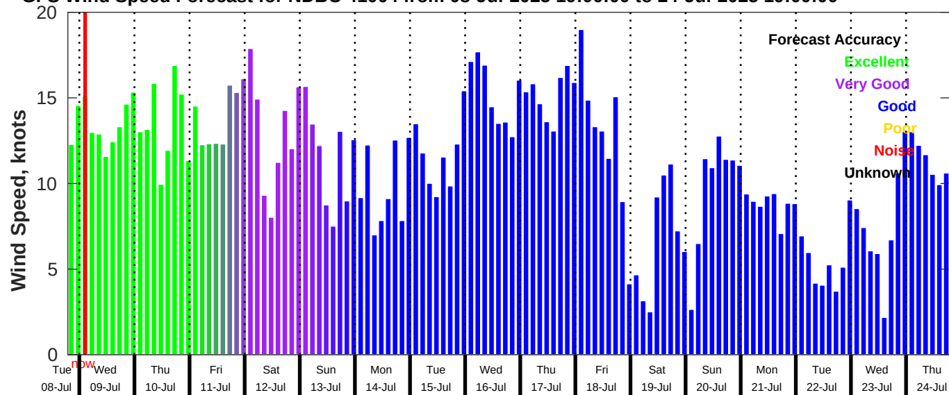
GFS Wind Speed Forecast for NDBC 41004 from 08-Jul-2025 19:00:00 to 24-Jul-2025 19:00:00
