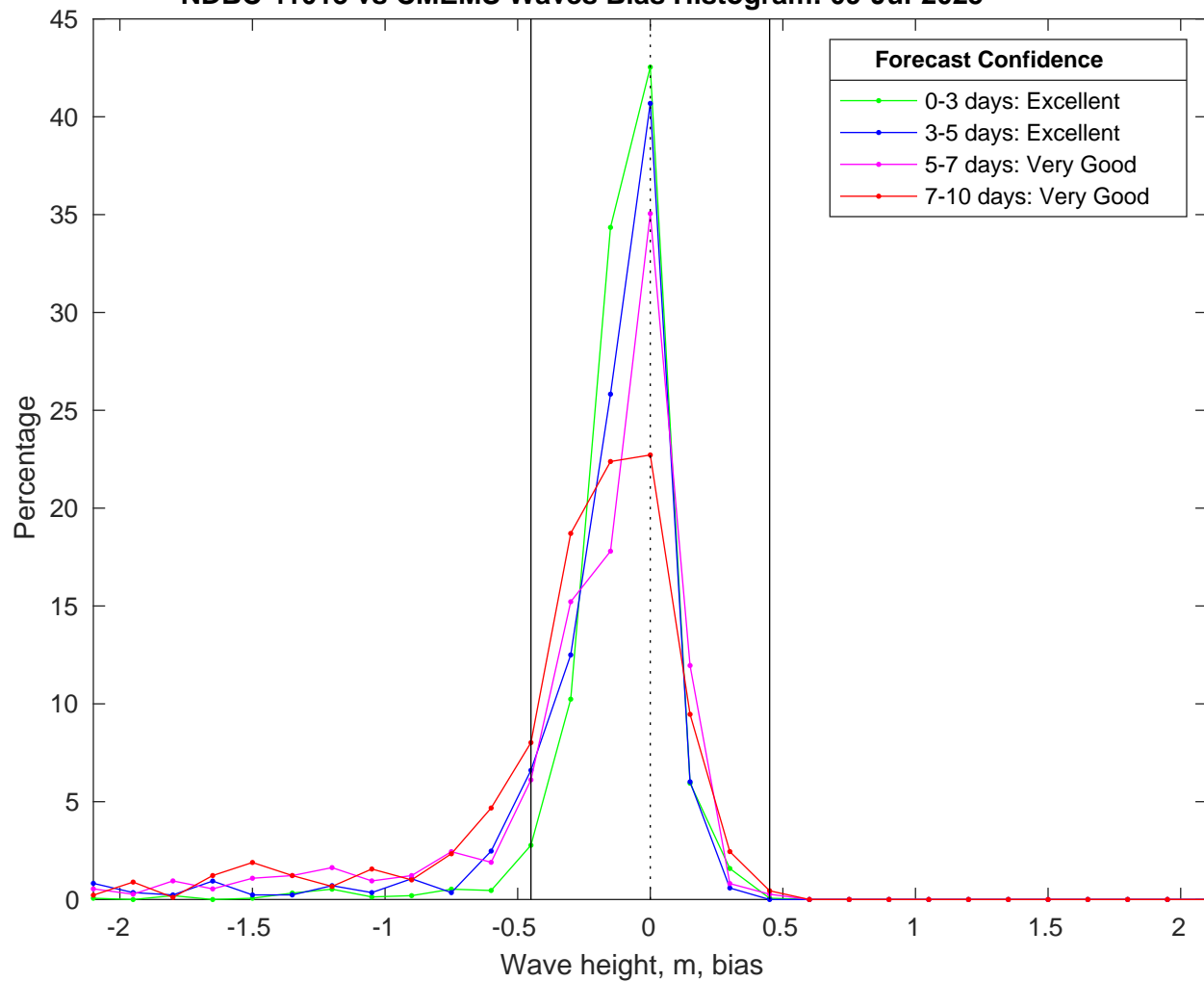
NDBC 41013 vs CMEMS Waves Bias Histogram: 09-Jul-2025
